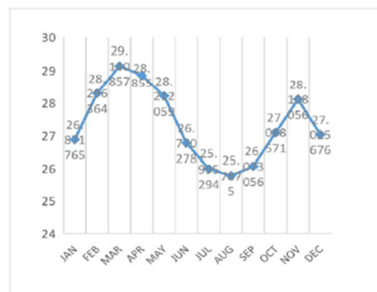
Figure 8: Monthly average temperature distribution of Yenagoa City
