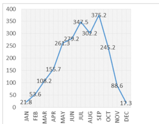
Figure 9: Monthly average rainfall distribution trend of Yenagoa City
