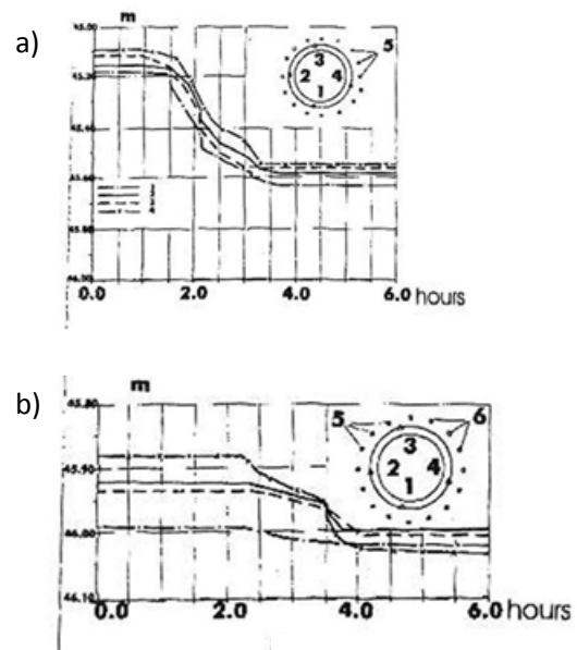
Figure 5: Electroosmosis deeping diagram phragments
