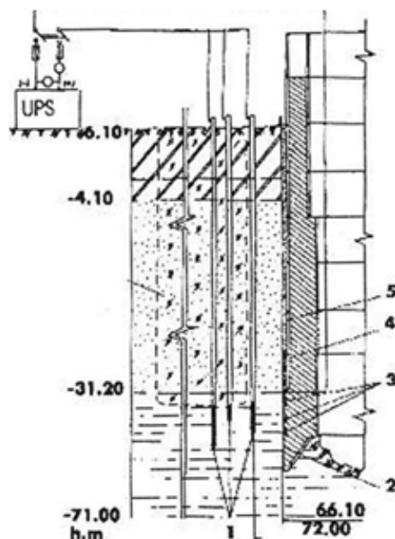
Figure 4: Scheme for electro osmosis edifice deeping
