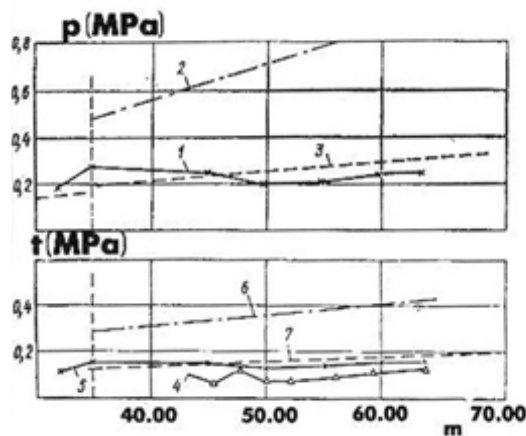
Figure 3: Pressure and friction measurements during the deeping process
