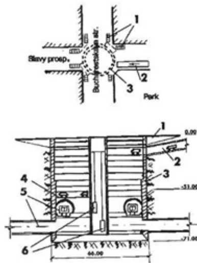
Figure 1: Multifunctional deep-set junction terminal (Location), (Junction terminal plan)
