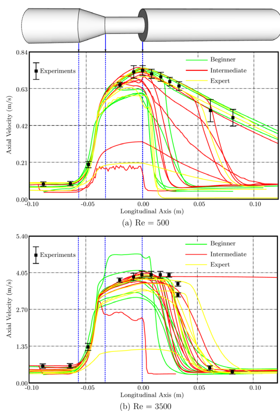
Figure 2: In the FDA study [1], the participants were requested to provide simulation data along the model centerline, among others. The results of the study for two Reynolds numbers, The graphs were re-created based on the data from [3]
