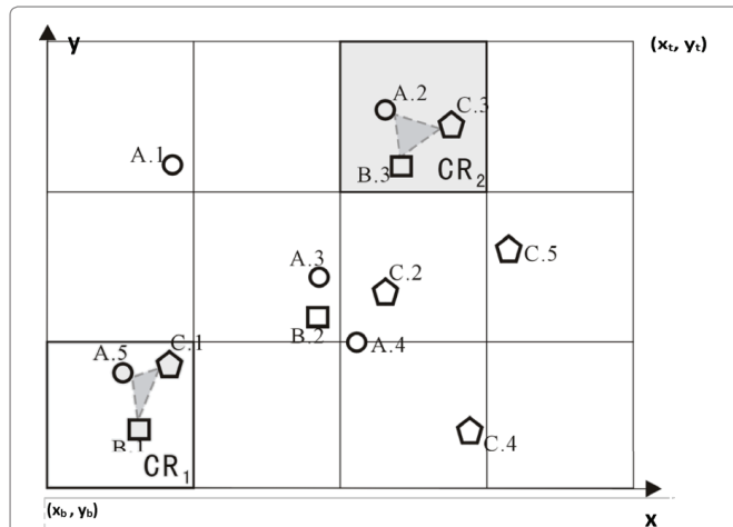
Figure 2: Co-ordinate representation of grid area showing right top corner (x_t, y_t) And left bottom corner (x_b, y_b) . The current location of the MO is (x_u, y_u)
