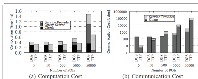
Figure 5: Comparisons of Computation and Communication costs of our proposed Direct Grid System (DGS) with the Trusted Third Party (TTP) architecture [1] in terms of number of points of interests (POI)
